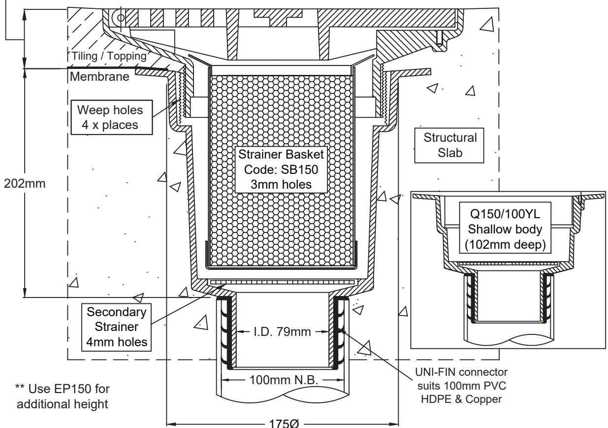
Typical Application
