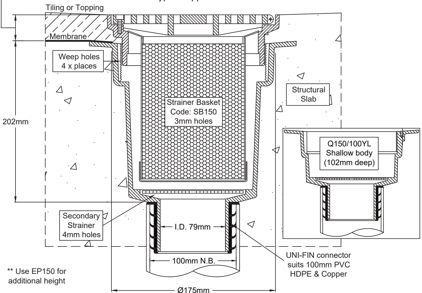
Typical Application
