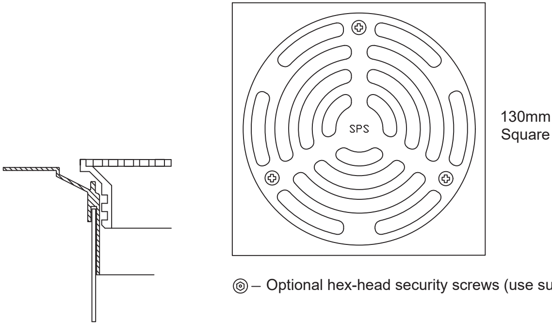
Installation with puddle flange
